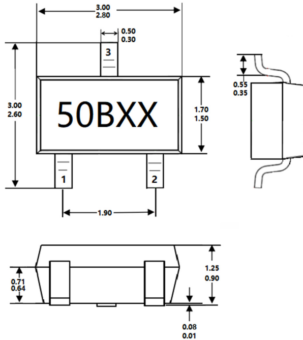
Package (SOT-23) (Top View)
